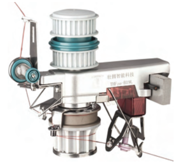
Positive Feeder THF20-B19L
